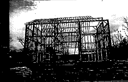
Partial skeleton of barn as of April '19
