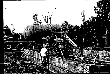
Pouring concrete for foundation
