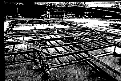
Bents prepped for raising
